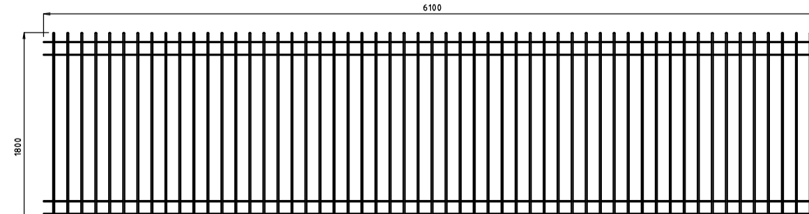
ANTOLEA - 100x110 - 25x6 - Ø12
